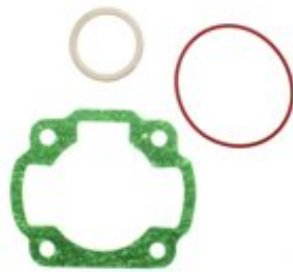
SSP-G 47mm 70cc 2-stroke Cylinder Gasket Set 169-189
