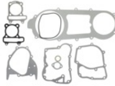
Universal Parts 150cc GY6 Long-Case Gasket Set 130-46
