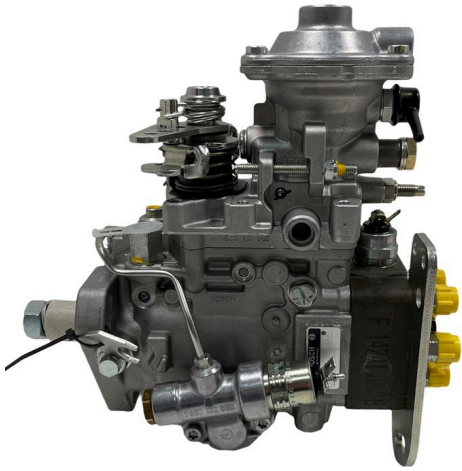
Bosch VE Dodge 5.9L
