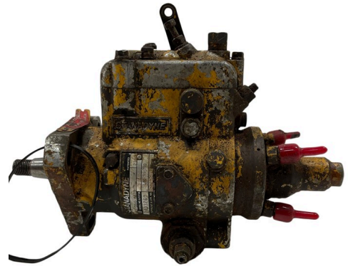
Stanadyne - Caterpillar / Perkins / Case (Agricultural & Industrial) DB2 & DB4
